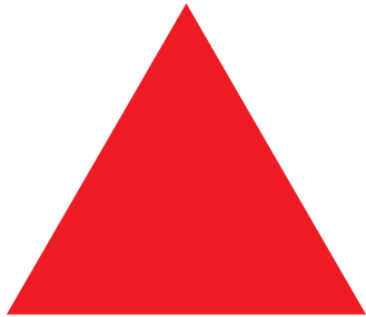
a regular triangle (called an equilateral triangle)
